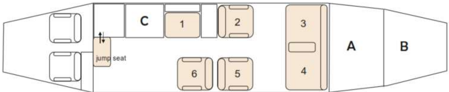
Configuration 1 - 6 seats
